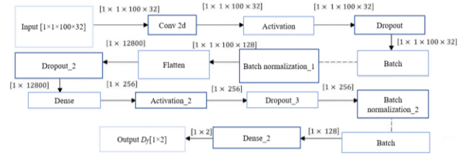
Figure 3. The structural design of DCNN.
