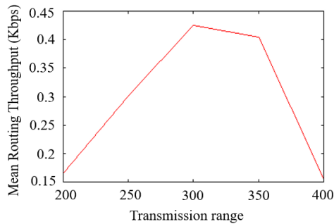
Figure 11. Average throughput variation based on transmission range (with calculated aggregation delay).
