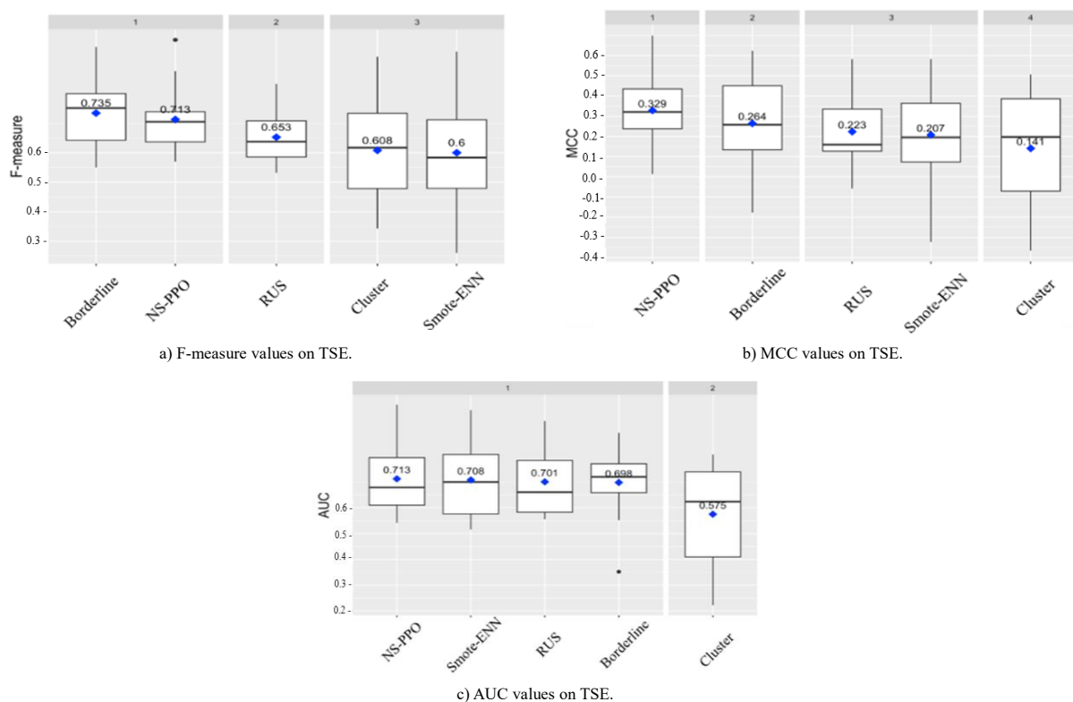
Figure 9. Performance and ESD test results of the NS-PPO and baseline methods on TSE.
