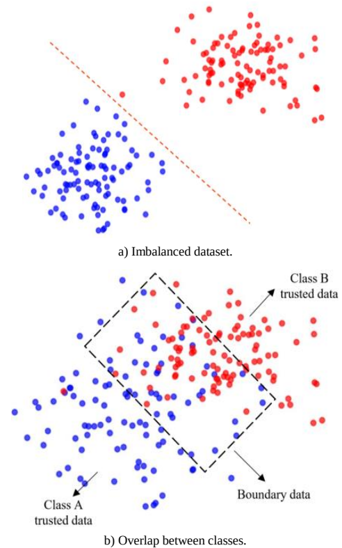
Figure 3. A comparative example of an ideal balanced dataset versus a dataset with the class overlap issue.
