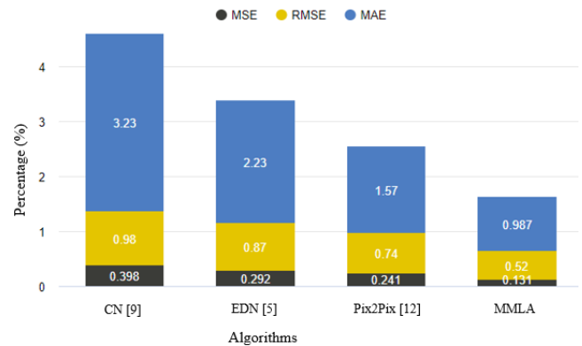
Figure 6. Comparison between algorithms based on reconstruction quality (conversion of chair).
