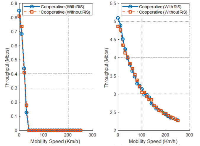
a) Throughput against mobility speed for 50 users at SNR of -20 dB. b) Throughput against mobility speed for 50 users at SNR of 20 dB.
