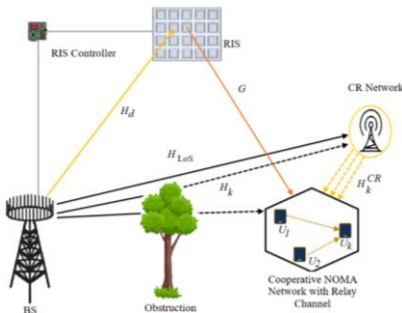
Figure 2. Illustrates mMIMO PD DL CR mMIMO cooperative NOMA with K users employing intelligent RIS and mmWave methodologies.
