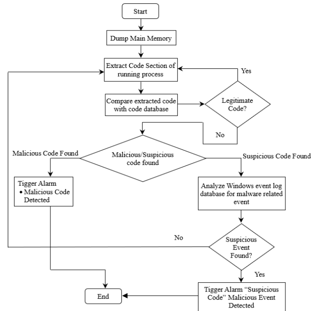
Figure 3. Flowchart of the proposed approach.
