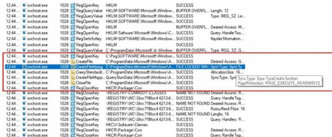
Figure 10. A screenshot of process monitor showing svchost.exe memory protection flags altered on 64-bit Window 10.
